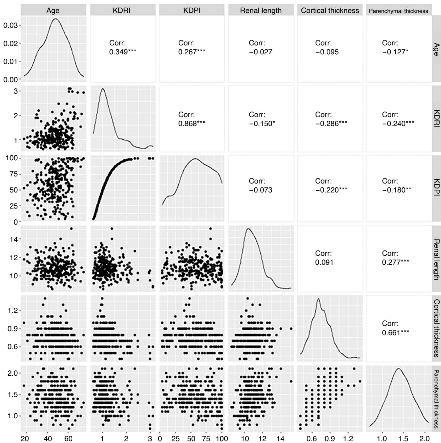
Supplementary Fig. 1. Scatterplot matrix of age, kidney donor risk index (KDRI), kidney donor profile index (KDPI), and ultrasound parameters.
